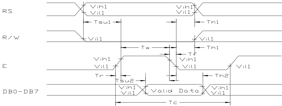
(2) Read mode(Reading data from KS0066 to Micom)
